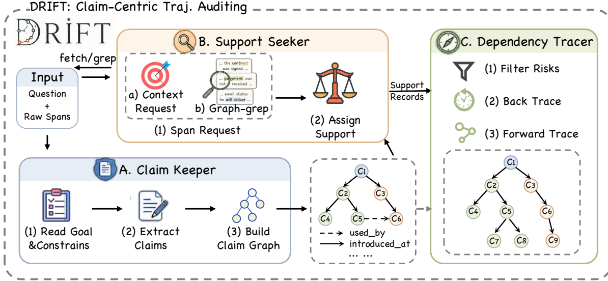
FIGURE 3 Overview of DRIFT: a claim-centric auditing workflow that builds trajectory-level claim ledgers, verifies support, and traces claim dependencies to localize first and follow-up errors.
