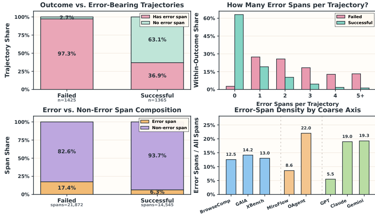
FIGURE 8 Basic error-burden statistics of annotated trajectories. We compare final failed and successful trajectories by whether they contain any annotated error span, the number of error spans per trajectory, the composition of error versus non-error spans, and the overall error spans density across benchmarks, frameworks, and model families.
