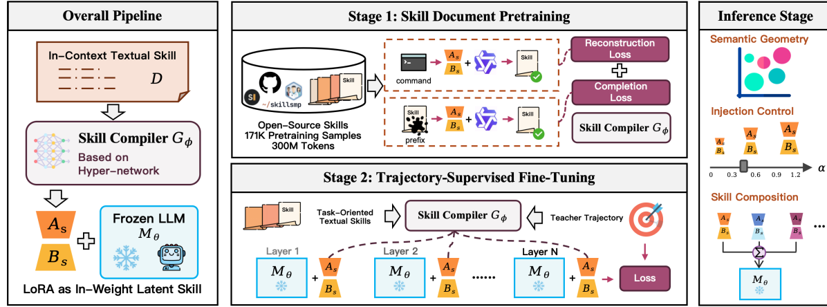
FIGURE 2 Overview of LatentSkill . Left: textual skills are transformed into in-weight latent skills through hypernetwork-based LoRA generation. Middle: the skill compiler is trained by skill document pretraining and trajectory-supervised fine-tuning. Right: the resulting latent skills support structured semantic geometry, controllable injection strength, and composable parameter-space arithmetic at inference time.
