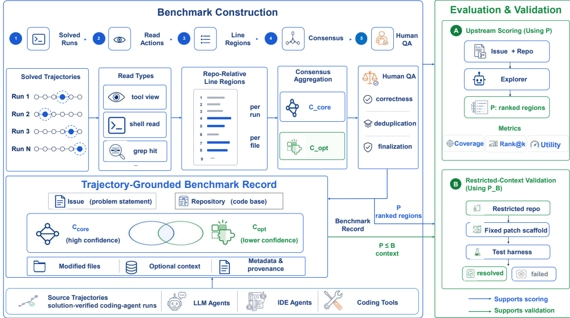
FIGURE 2 Overview of SWE-Explore. From solution-verified trajectories, SWE-Explore extracts read actions, aggregates them into core and optional context, and evaluates explorers using both upstream exploration metrics and downstream restricted-context validation.
