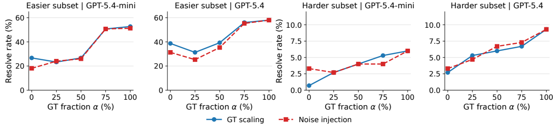
FIGURE 5 Resolve rate as the visible context degrades from the Oracle’s full core set R_{\text{core}} to either \alpha\% of R_{\text{core}} alone ( GT scaling , solid) or \alpha\% of R_{\text{core}} padded back to full size with random non-core regions ( noise injection , dashed).
