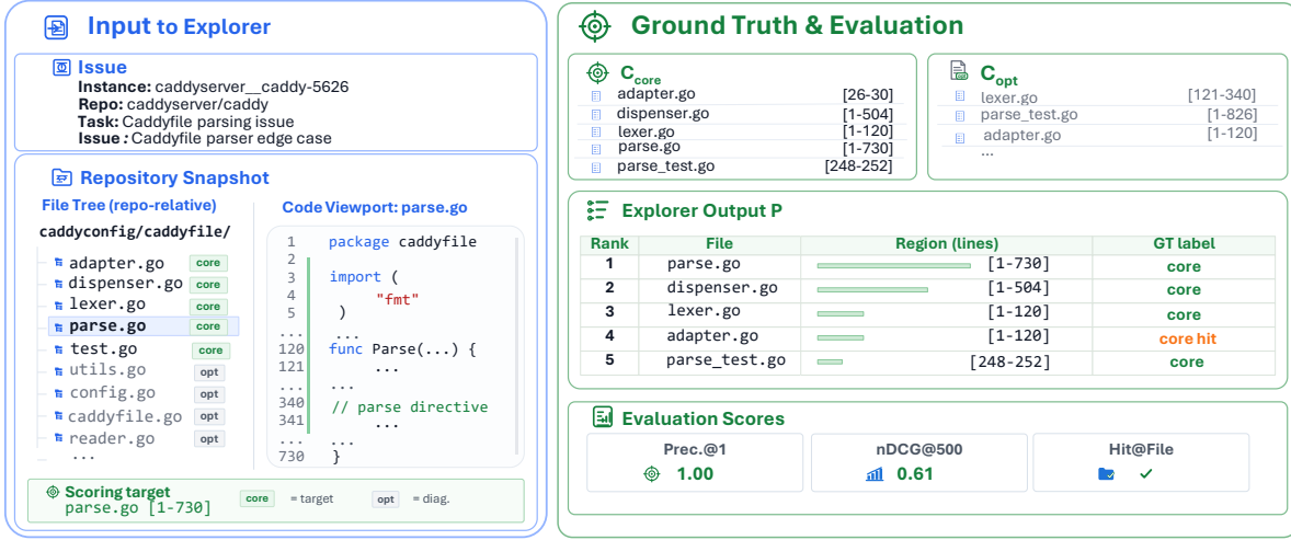
FIGURE 4 Example of a SWE-Explore instance. Left: an issue plus a repo snapshot with the highlighted core span. Right: trajectory-derived core regions C_{\text{core}} (scoring target) and optional regions C_{\text{opt}} , an explorer’s ranked prediction scored against C_{\text{core}} .
