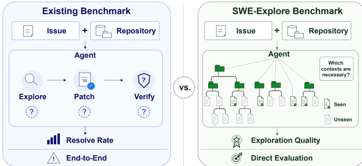
FIGURE 1 Motivation of SWE-Explore. A holistic metric of resolution rate conflates exploration, localization, and patch synthesis. SWE-Explore isolates repository exploration as a line-level evaluation target.
