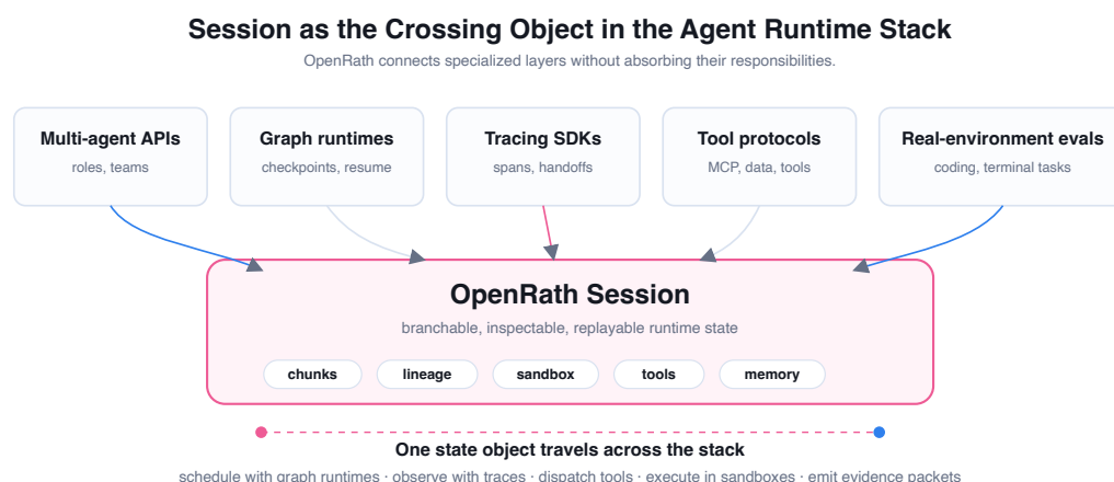
FIGURE2 OpenRath’s ecosystem role is a crossing-object boundary. It can work with specialized agent APIs, graph runtimes, tracing SDKs, tool protocols, sandbox providers, and evaluation harnesses by making their effects visible in one Session .
