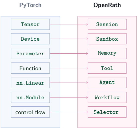
FIGURE 3 The PyTorch lens. Each agent-runtime concern maps onto one OpenRath object, with Session as the flowing value (the tensor of the runtime) and Selector routing control flow at run time. The mapping is a teaching device, not a claim that agent systems are neural networks.
