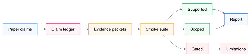
FIGURE 7 Claim-to-evidence protocol: report claims pass through a ledger, evidence packets, and a smoke suite before becoming supported text, scoped text, or explicit limitations.
