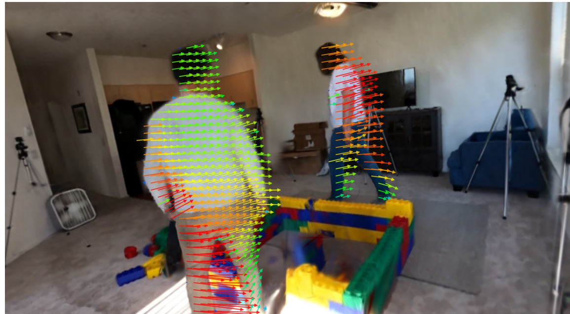
Backward optical flow F_{t \rightarrow t-1-i}
