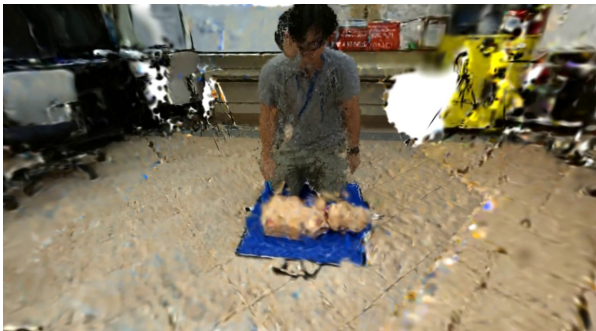
MonoFusion
