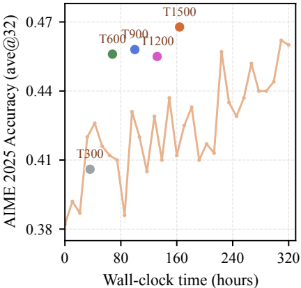
Wall-clock-matched AIME 2025
