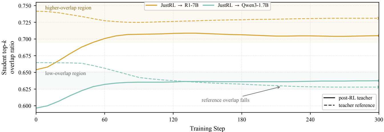
JustRL overlap dynamics
