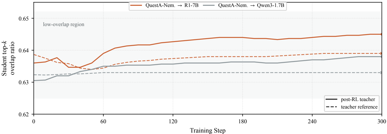
QuestA-Nemotron overlap dynamics
