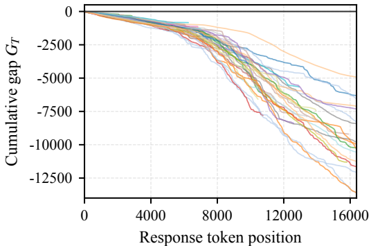
Qwen3-1.7B: 64 rollouts
