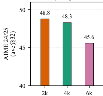
Validation @ step 40
