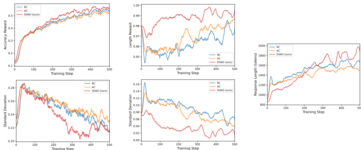
FIGURE 2 Training dynamics on Qwen3-8B-Base . Left: accuracy reward (top=mean, bottom=std). Middle: length reward (top=mean, bottom=std). Right: average response length.
