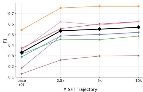
FIGURE 4 Effect of the number of SFT trajectories on F_1 scores (EM is in Figure 17 in Appendix C) after RL training.
