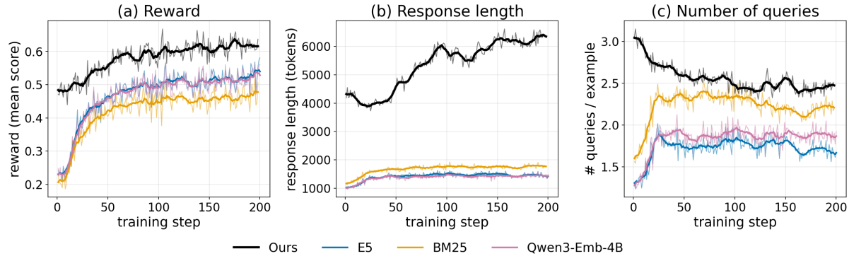
FIGURE 5 Training dynamics over 200 steps comparing GrepSeek with retrieval baselines (E5, BM25, and Qwen3-Emb-4B). (a) Mean reward score during training. (b) Average response length measured in tokens. (c) Average number of search queries generated per example.
