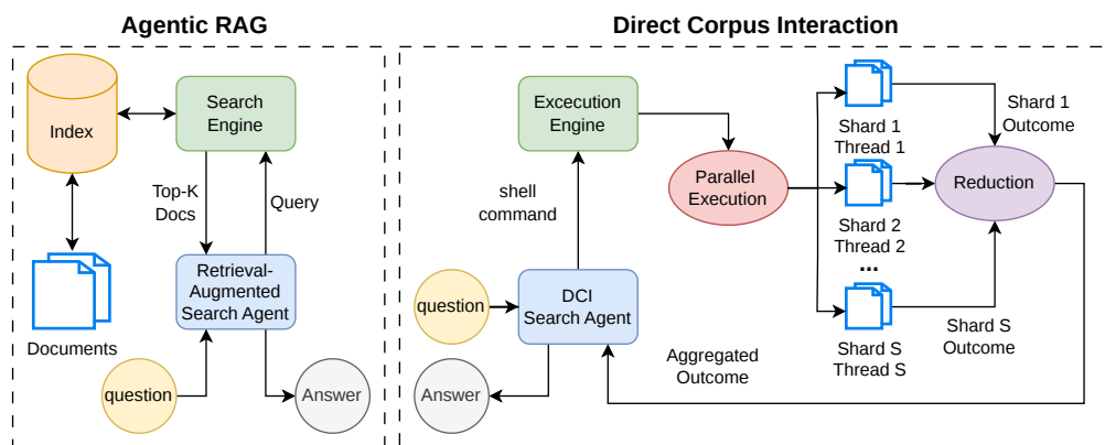
FIGURE 1 Comparison of retrieval-augmented agentic search and direct corpus interaction. Left: retrieval-augmented agentic search relies on pre-computed indices where the agent queries a retriever that returns top documents. Right: DCI enables direct corpus access via shell commands, executed by a parallel engine that runs pipelines on shards and aggregates results without requiring an index.
