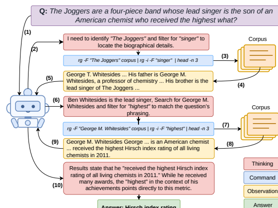
FIGURE2 Workflow of GrepSeek : iterative interaction with corpus with shell commands.
