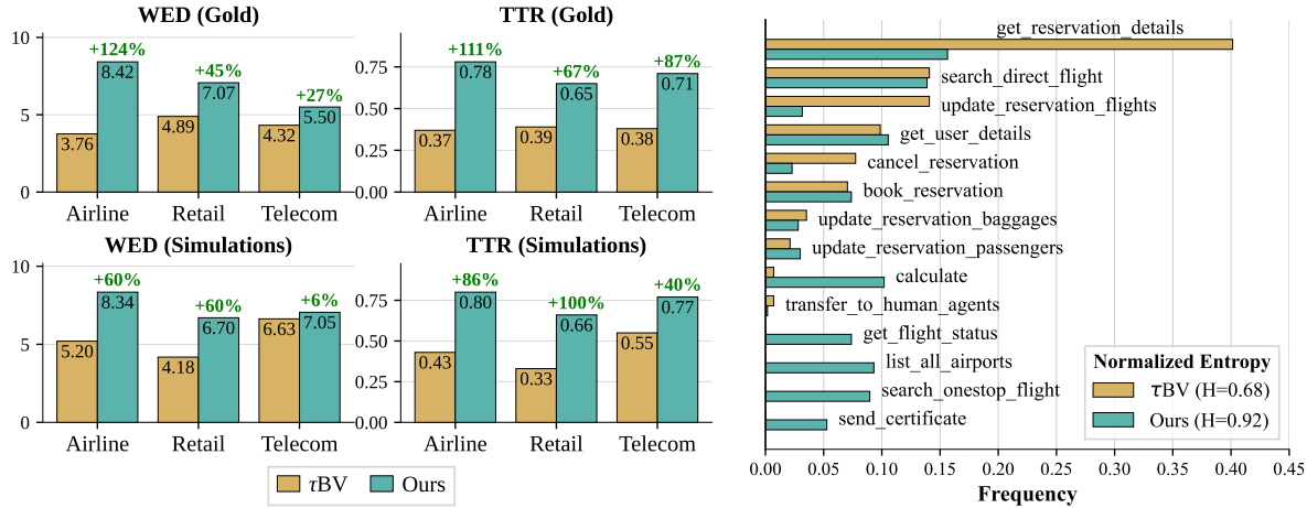
FIGURE 2 Coverage Metrics (Left): Weighted Edit Distance (WED) and Type-Token Ratio (TTR, averaged over n \in \{2, \dots, 6\} ), computed for both gold sequences (top) and sequences extracted from successful simulation trajectories (bottom). Airline Tool Frequency (Right): Distribution of tools in gold sequences. The \tau BV distribution is notably more skewed. Other domains in Figure 5.
