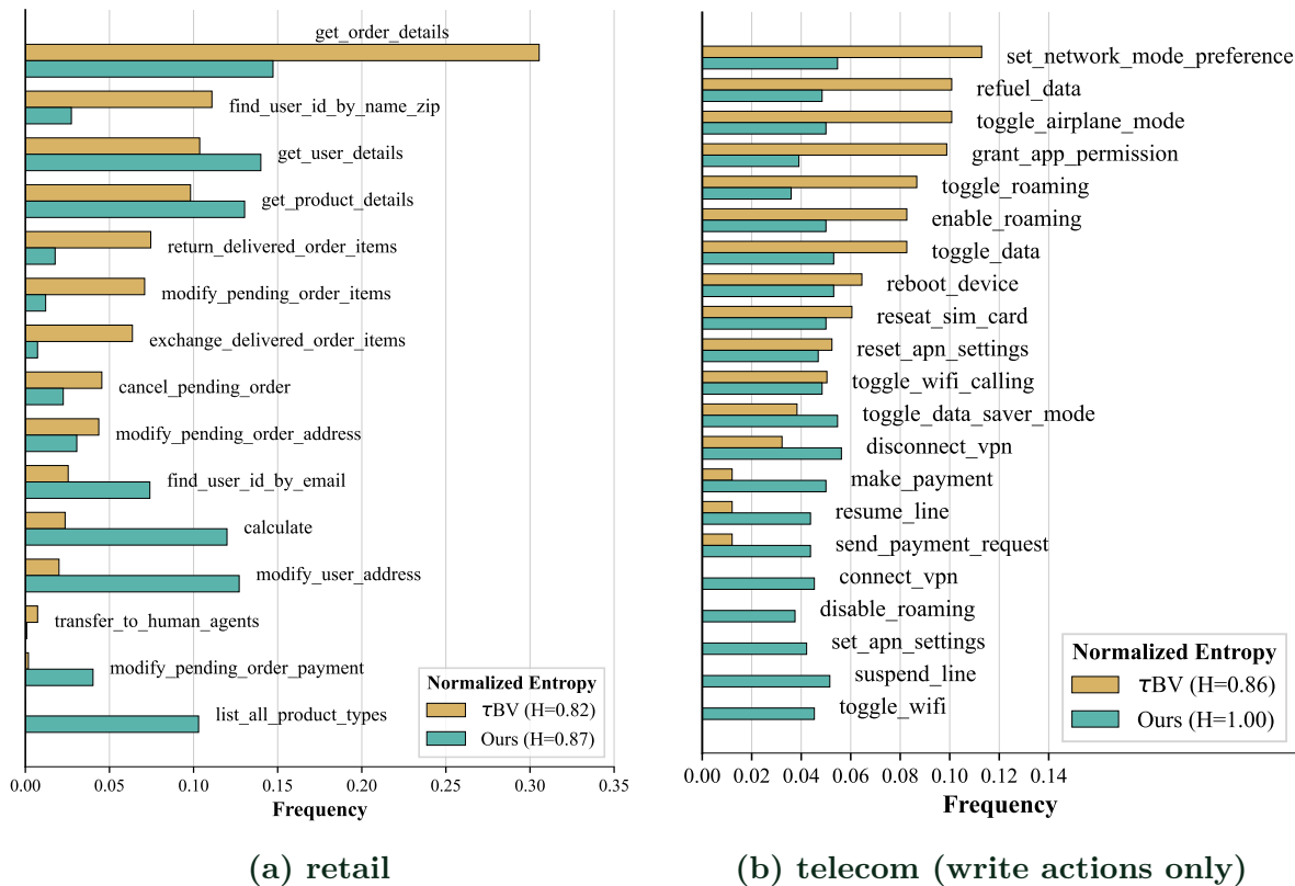
FIGURE 5 Per-tool relative frequency on the retail and telecom domains, comparing \tau BV against \tau^c -Bench; the airline counterpart is in Figure 2. Normalised entropy H is reported in each panel’s legend; tools are ordered within each panel by \tau BV task frequency. Telecom is restricted to write actions (21 of 43 tools, both distributions re-normalised over this subset) since the \tau BV telecom tasks does not include read tools in their gold tool sequences.
