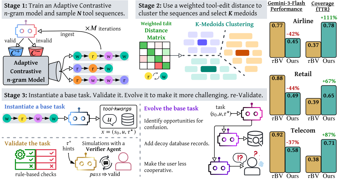
FIGURE 1 Illustration of TASTE, our three-stage method for synthetic task generation. We demonstrate the method across the three domains of \tau^2 -Bench (Verified, \tau BV). Evaluating a Gemini-3-Flash agent (averaged over two different user LLMs) shows that, unlike \tau BV, \tau^c -Bench is non-saturated. Besides being more challenging, \tau^c -Bench exhibits broader coverage, requiring agents to exercise a more diverse set of tool combinations, as quantified by the type-token ratio (TTR; see §5).
