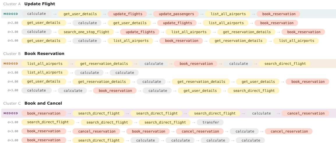
FIGURE 7 k -medoids clusters on the airline domain under weighted edit distance (a) vs. unweighted edit distance (b). Each cluster shows its medoid (top row) and three nearest neighbors; chips are colored by tool type (READ, WRITE, GENERIC).
