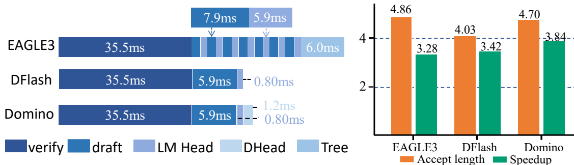
FIGURE 1 Latency breakdown and performance comparison on Qwen3-8B under a 16-token speculative decoding budget. Left: per-step latency breakdown measured on an A100 GPU with context length 1024, where Verify denotes the target-model verification latency and Draft denotes the draft-model forward latency. LM Head , DHead , and Tree denote the output projection, Domino head, and tree construction/sampling overheads, respectively. Right: acceptance length and end-to-end speedup evaluated on GSM8K. All three draft models are trained on the same dataset.
