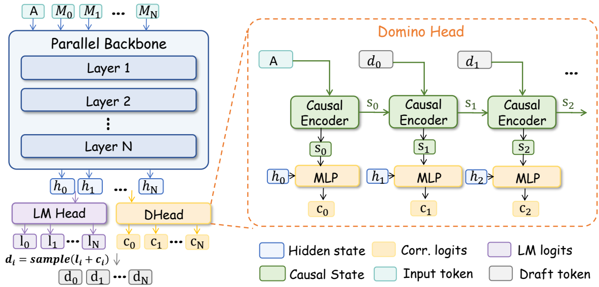
FIGURE 3 Overview of Domino. The parallel backbone produces hidden states for the whole draft block in one forward pass. The Domino head sequentially updates a causal state from previously sampled draft tokens and generates correction logits c_i , which refine the base logits l_i . Each draft token is sampled from the final logits l_i + c_i .
