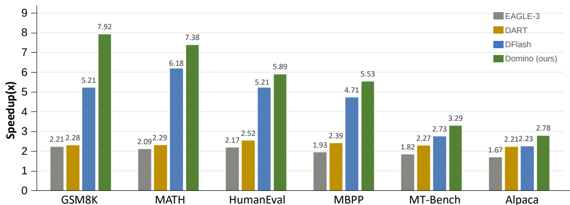
FIGURE 2 Speedup comparison of Domino, DFlash, and EAGLE-3 relative to autoregressive decoding on Qwen3-8B using the Transformers backend.
