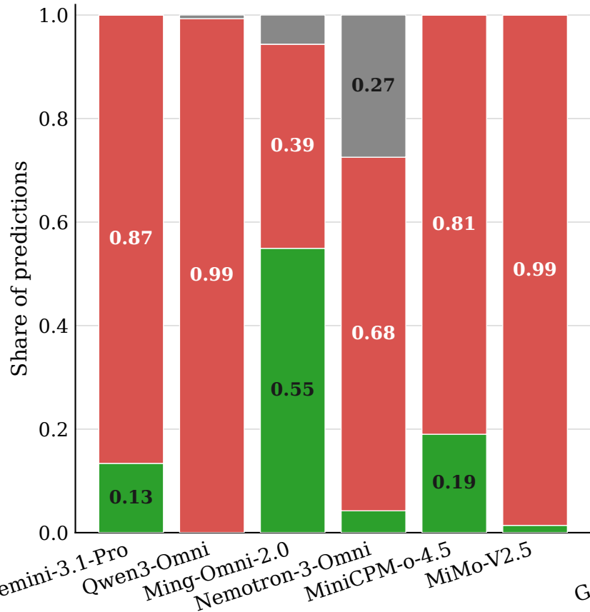
Mute task
