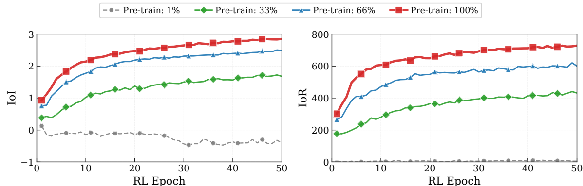
FIGURE 6 The impact of pre-training maturity on reinforcement learning efficiency. We evaluate the performance of ProRL across different stages of the pre-training process (1%, 33%, 66%, and 100% completion) on the MovieLens-1M dataset. The results indicate that a sufficiently converged semantic prior is a prerequisite for effective RL optimization, as it effectively constrains the action space and mitigates the sparse reward challenge in proactive guidance.
