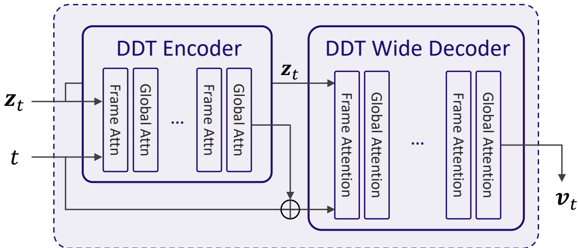
(c) GARD Denoiser Architecture
