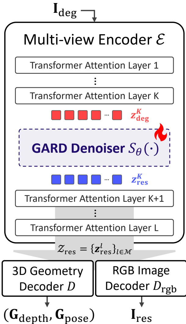
(a) GARD Framework
