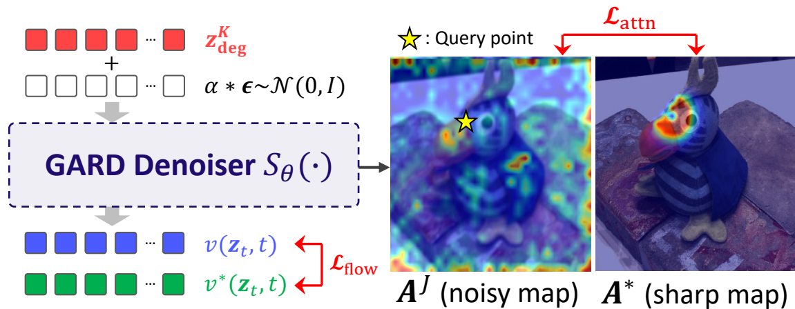
(c) GARD Denoiser Architecture
