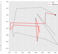
FMA-Net
