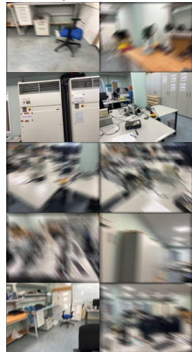
Input Views
