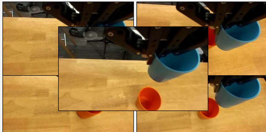
Multi-view Inputs
