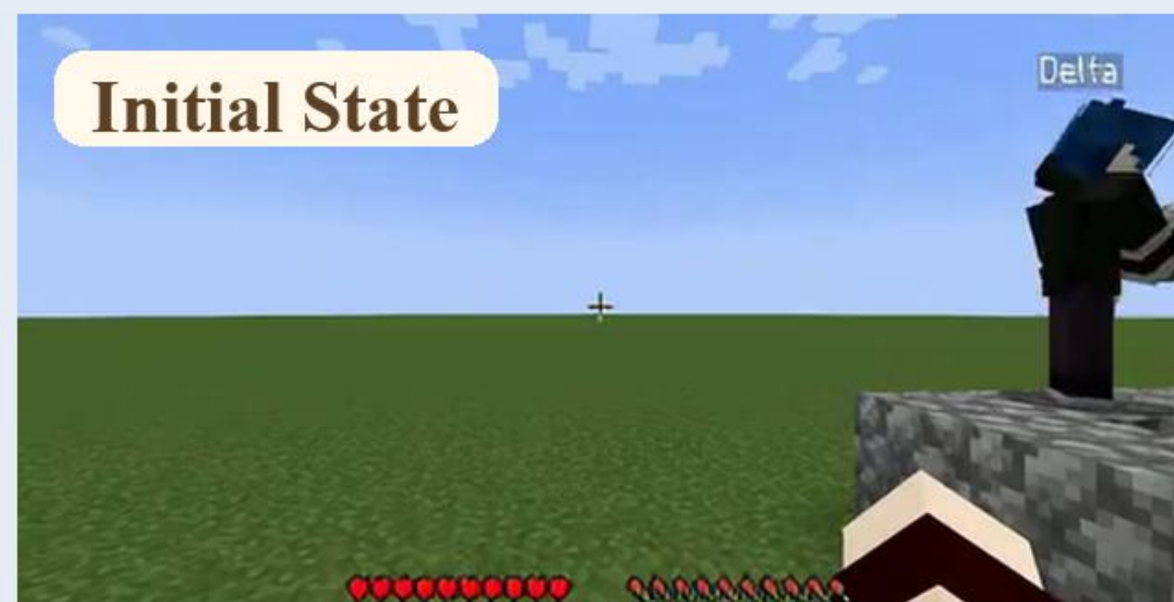
Agent 2
