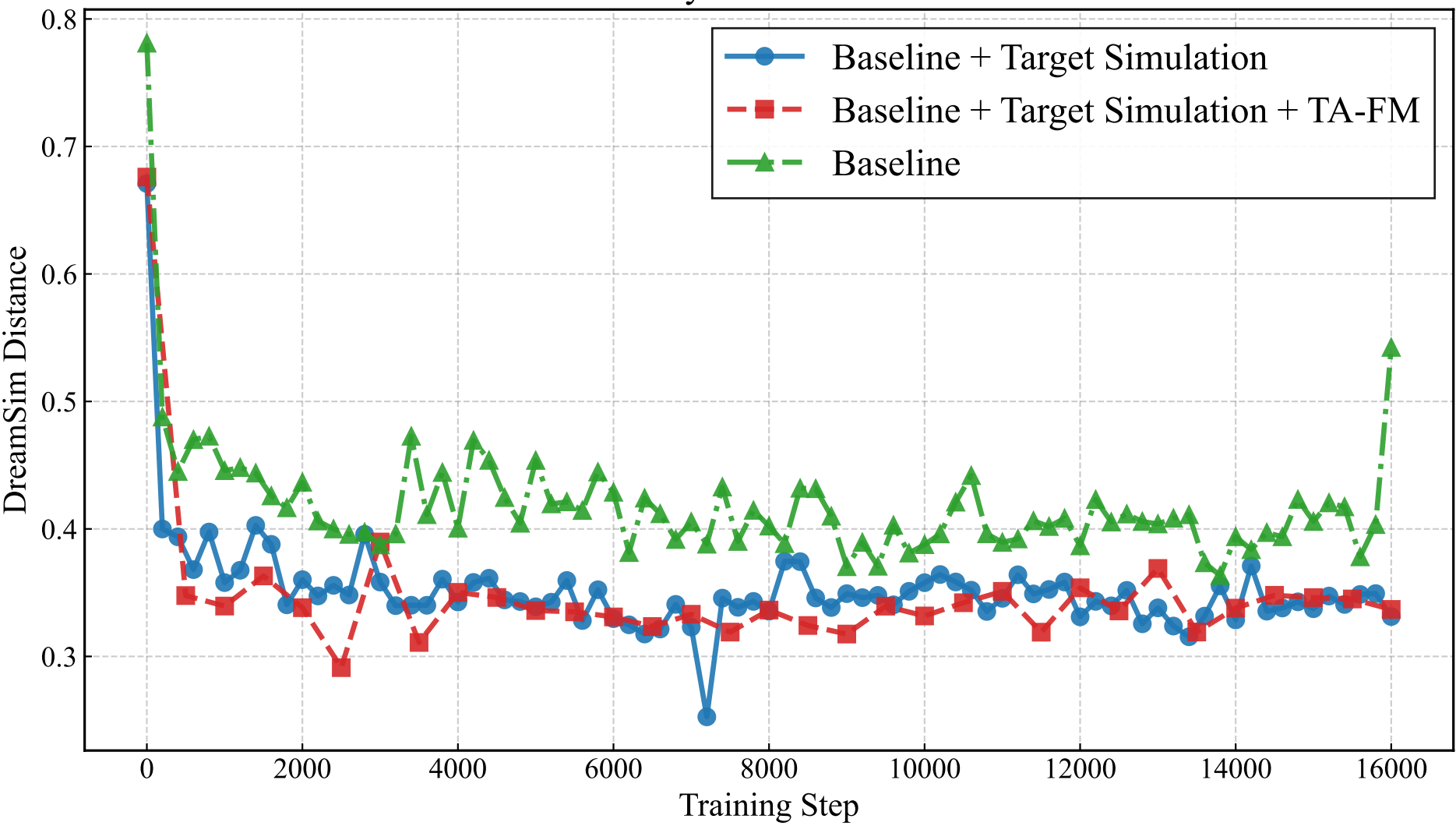
Ablation Study on DreamSim Distance
