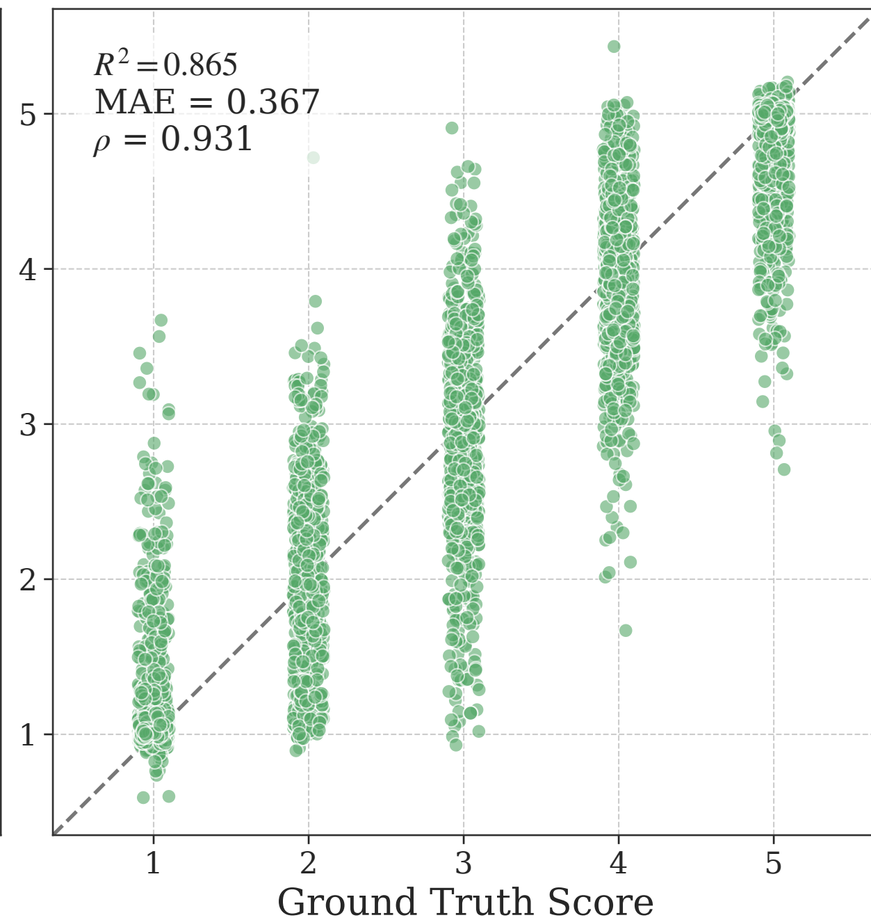
Recording Quality
