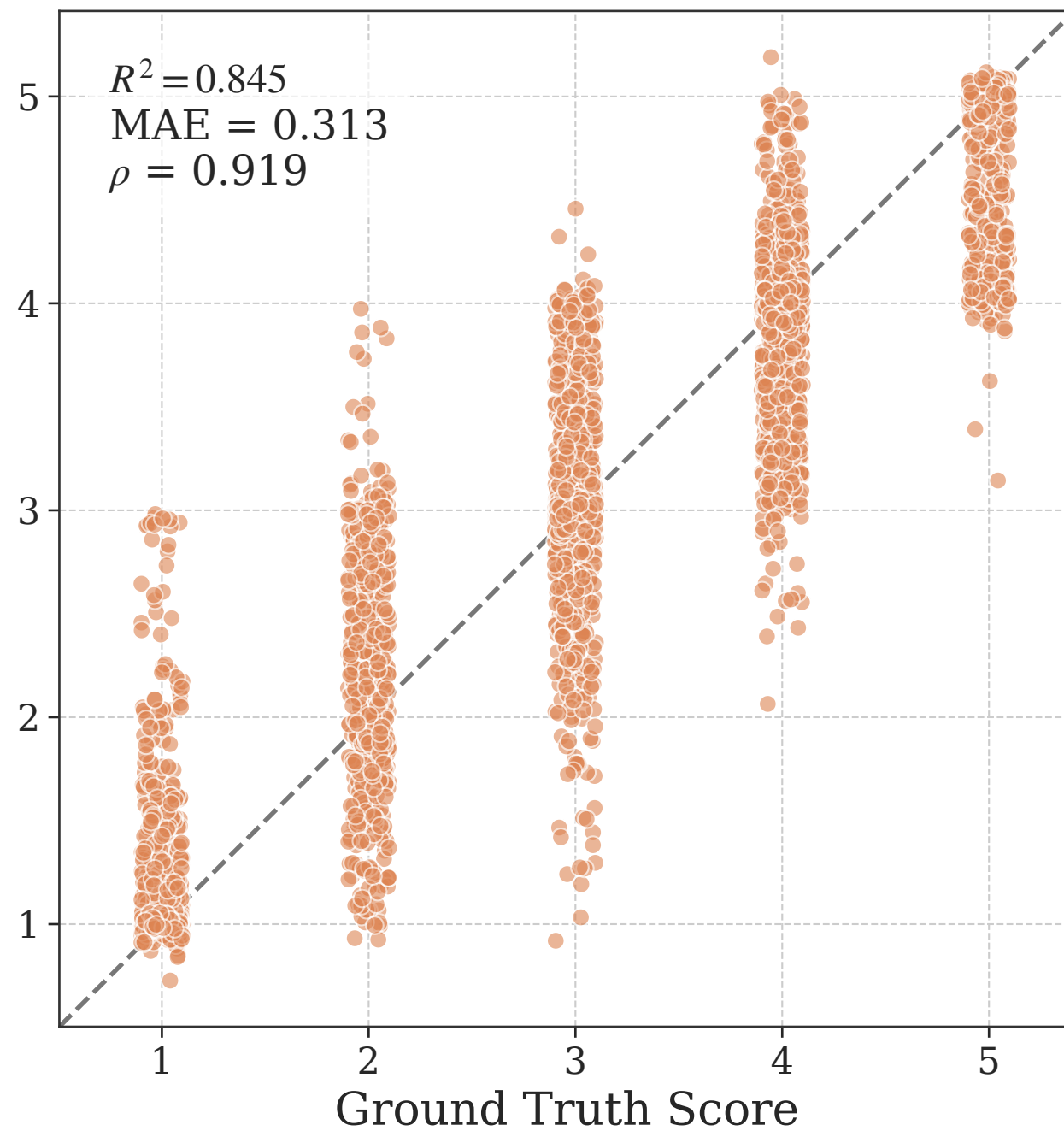
Instruction Clarity
