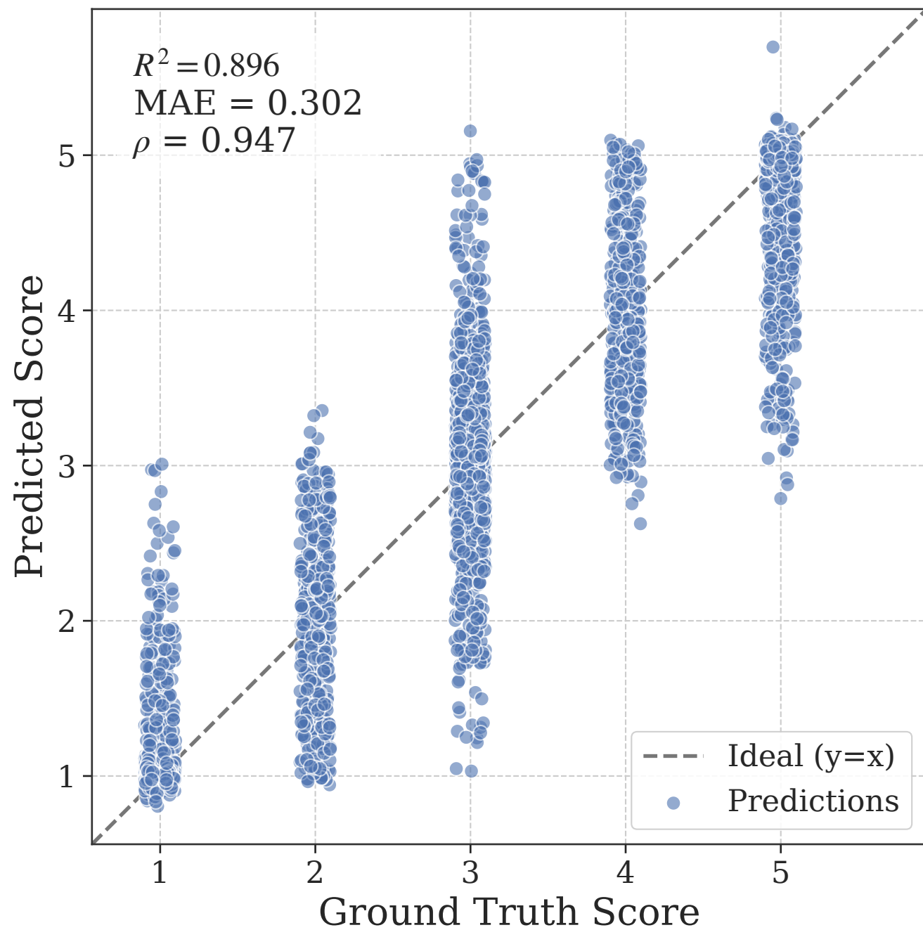
Topic Relevance
