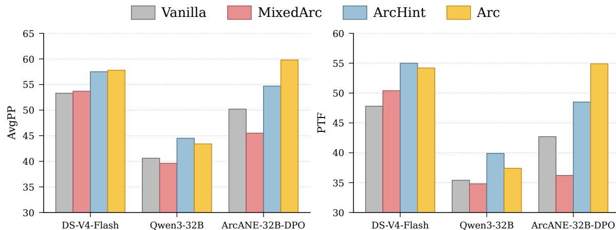
FIGURE 4 Arc source-of-effect ablation across three models, validated subset. DS refers to DeepSeek.
