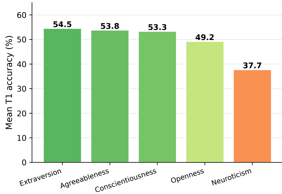
(a) Per-trait T1 accuracy (mean over 27 models)
