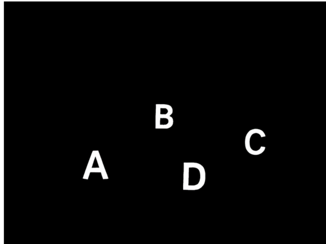
SenseNova-Vision
