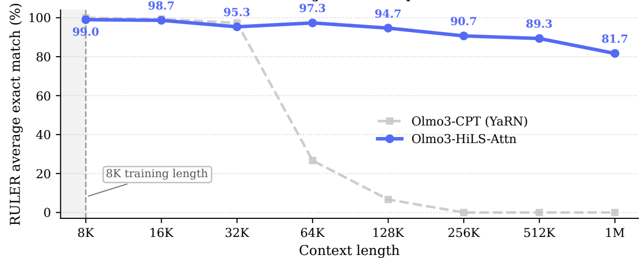
RULER Long-Context Extrapolation
