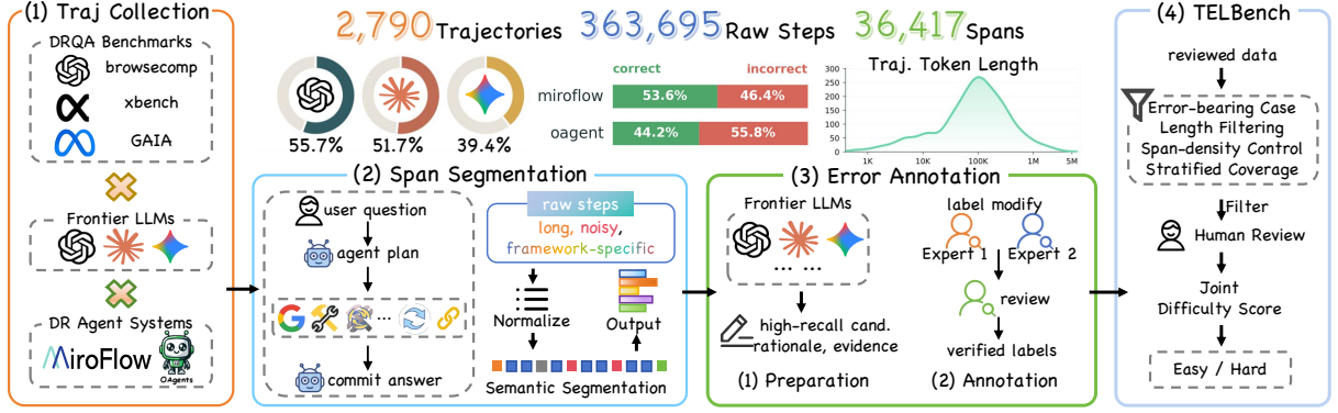
Figure 1: Data curation pipeline for TELBENCH, covering trajectory collection, log normalization, semantic-span segmentation, LLM-assisted candidate labeling, and expert-verified error annotation.
