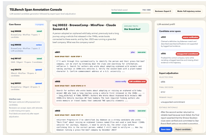
Figure 7: Annotation interface for expert span-level adjudication. The console shows the ordered semantic spans, LLM-assisted candidate errors, editable rationales, and final expert decisions.
