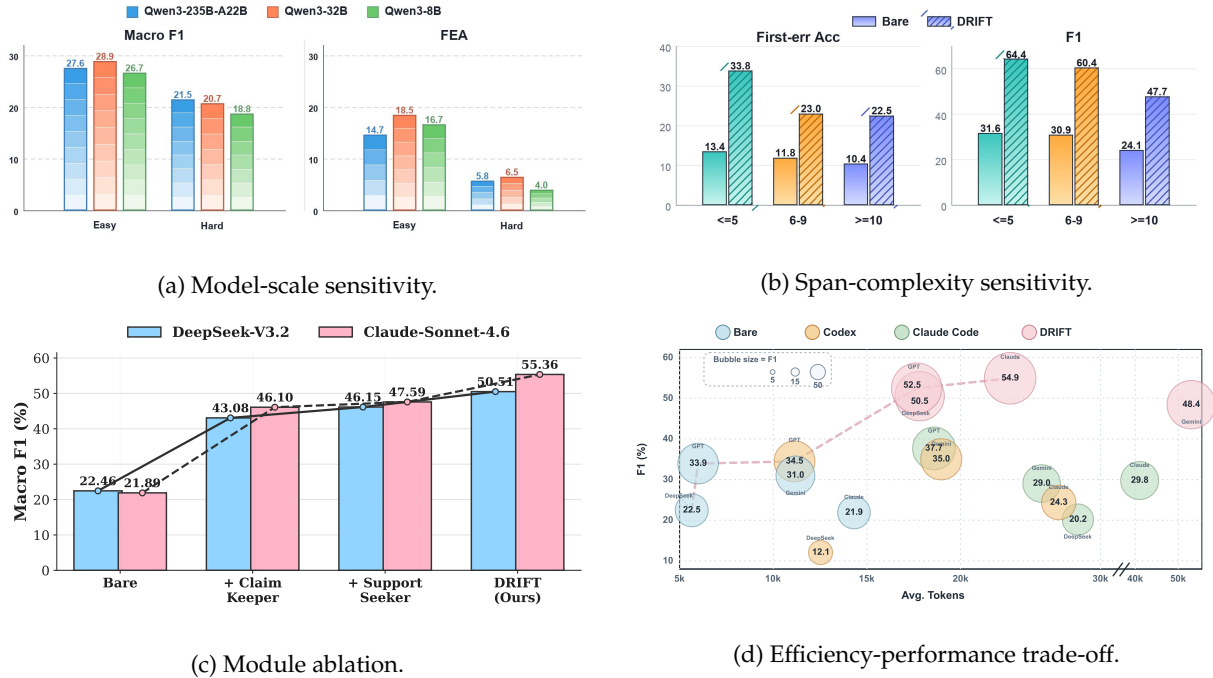
Figure 5: Further analysis of DRIFT. We examine robustness across model scale and span complexity, then verify that the gains come from the proposed modules and remain competitive under token cost.
