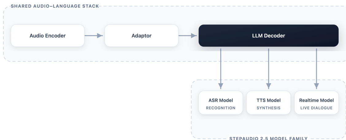
FIGURE 1 A unified view of the StepAudio 2.5 model family. The shared audio-language stack provides the common architectural basis used to organize ASR, TTS, and Realtime, while the three systems serve different deployment goals.
