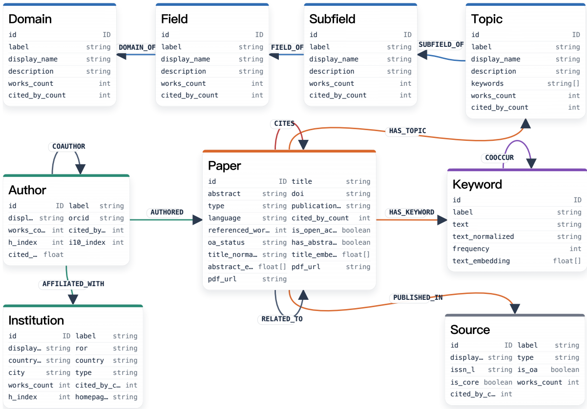
FIGURE 2 Schema of SciAtlas. By integrating 9 kinds of entity nodes and 12 kinds of relational edges, SCIATLAS provides a structured topological cognitive substrate that dismantles disciplinary barriers and furnishes AI agents with a global perspective. The complete schema (including entities, relations, attributions) of SCIATLAS can be found in Appx.A.
