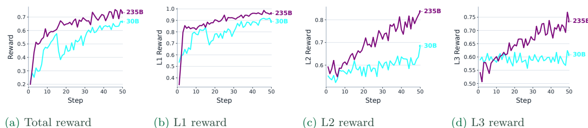
FIGURE 6 Reward trajectories during GRPO training. We track the total reward together with its L1, L2, and L3 components for Macaron-A2UI-30B and Macaron-A2UI-235B over training steps. The L1 reward rises first and most rapidly, while L2 and L3 improve more gradually. Higher is better.
