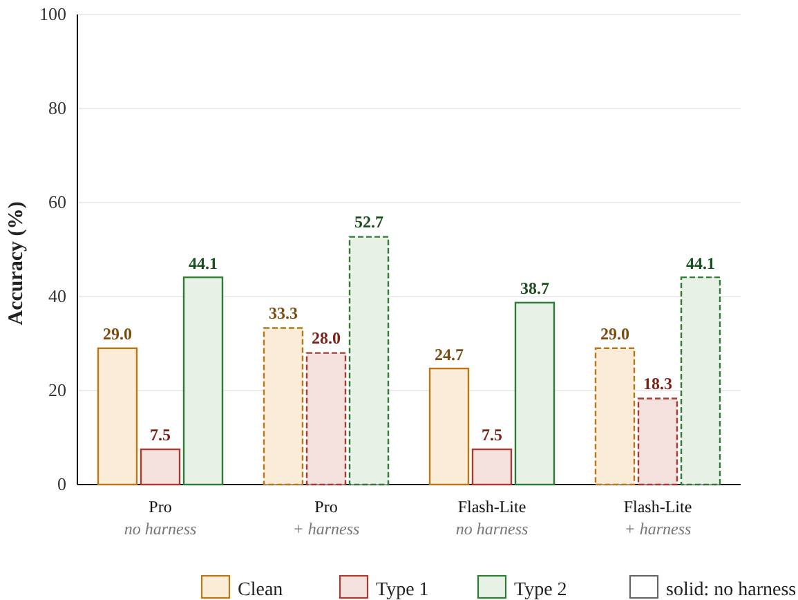
(a) Accuracy
