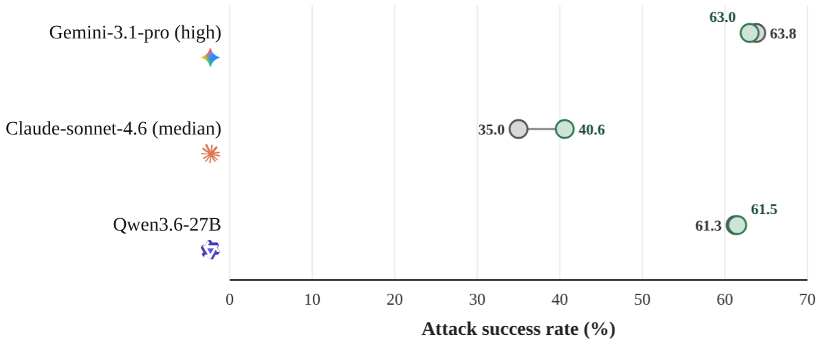
Panel A — Type 1 ASR
