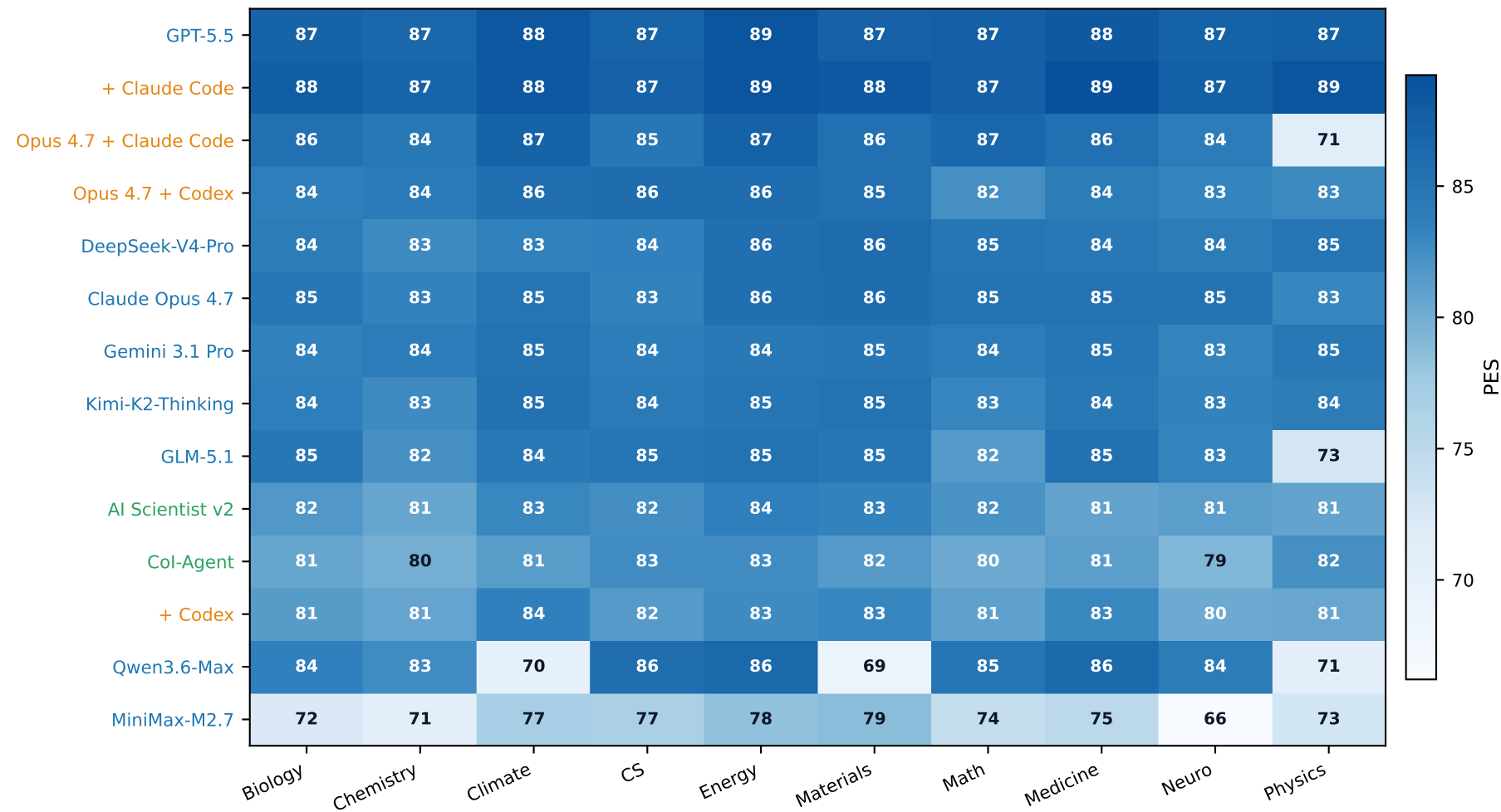
Lineage-setting PES by domain
