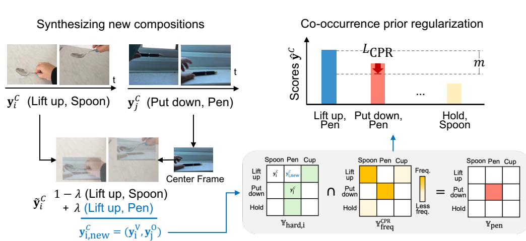
(b) Co-occurrence Prior Regularization
