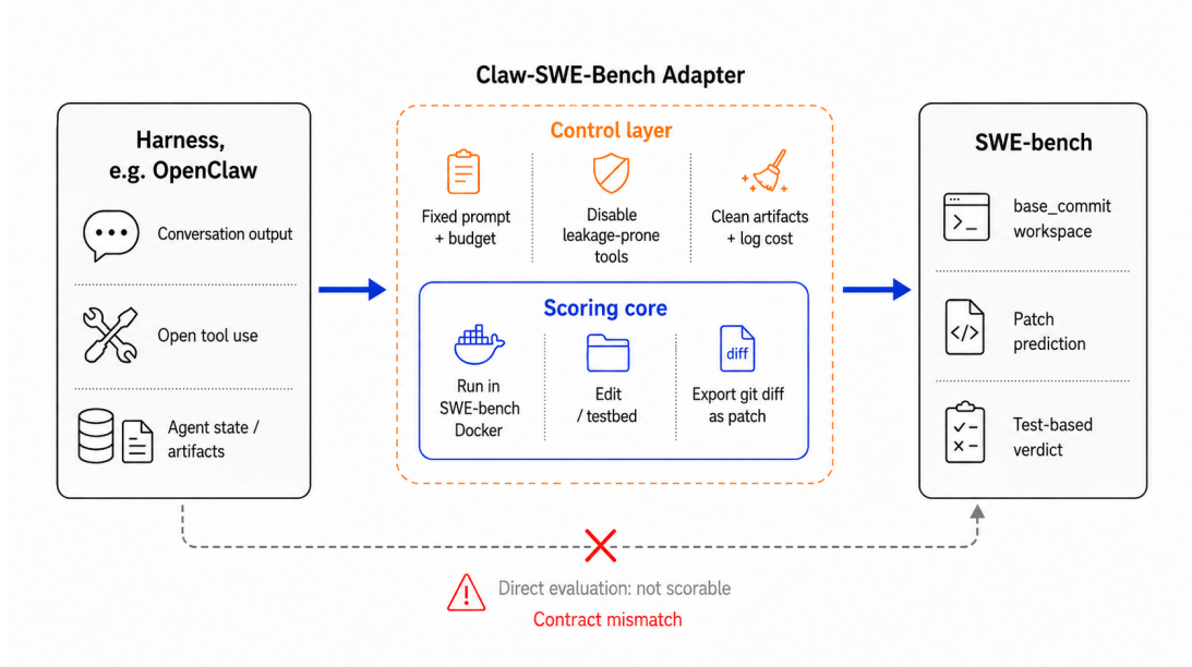
Figure 2. Contract mismatch between OpenClaw-style harnesses and SWE-bench. The adapter converts a general agent interaction into a SWE-bench-scored patch prediction, while outer controls ensure fairness, comparability, and traceable cost.
