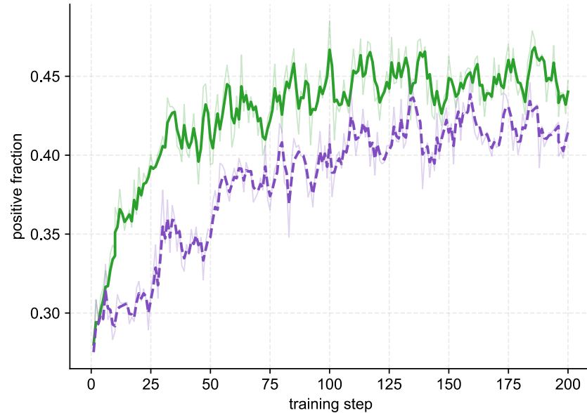
Fraction of Positive Advantages
