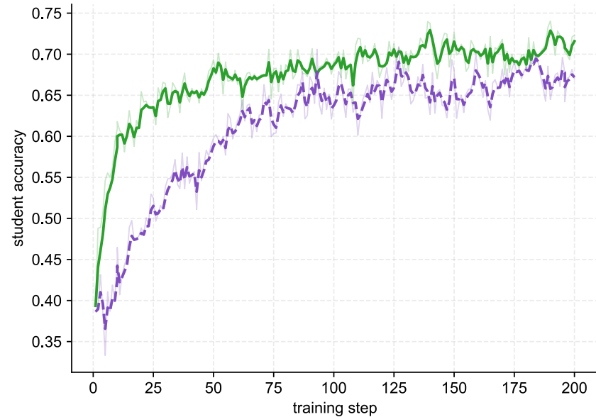
Student Accuracy
