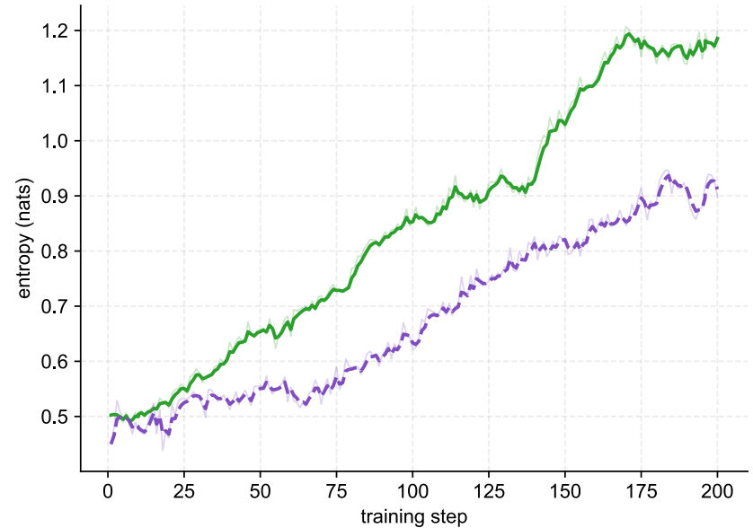
Shannon Entropy
