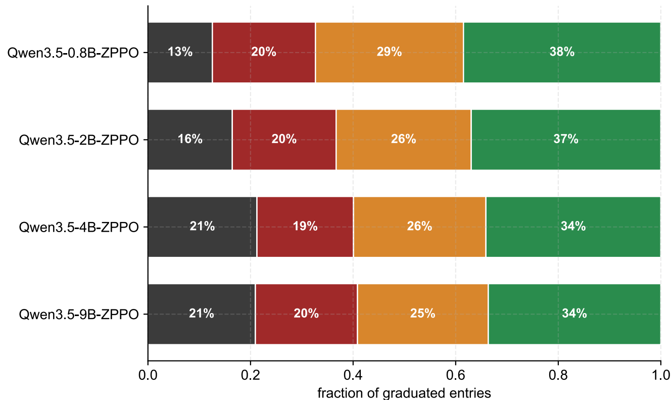
Graduation composition by Entry Rollout Accuracy at Admission (per-model %)
