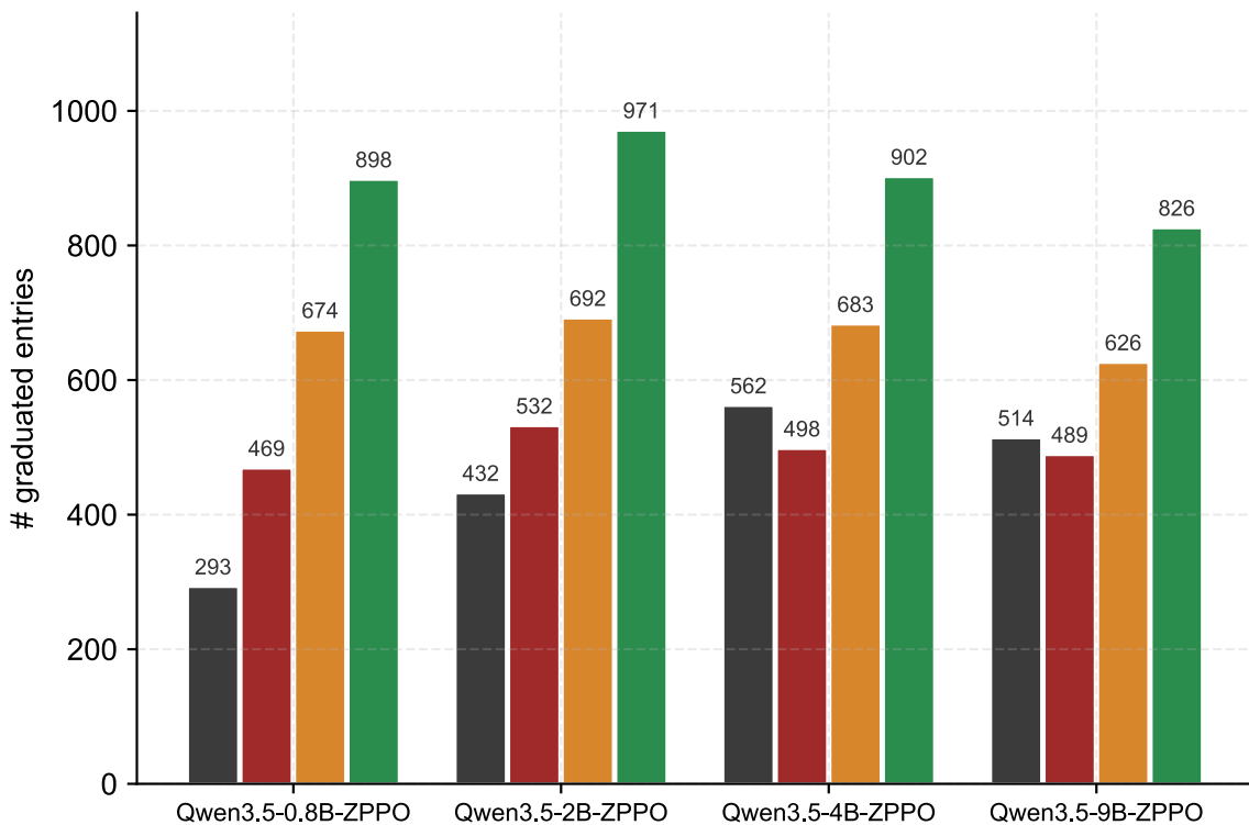
Graduations by Entry Rollout Accuracy at Admission (counts)
