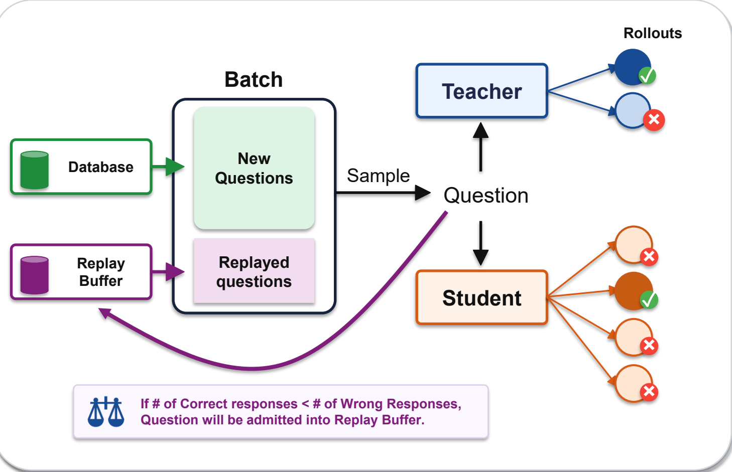
(a) Rollouts and Hard Question Admission to Replay Buffer
