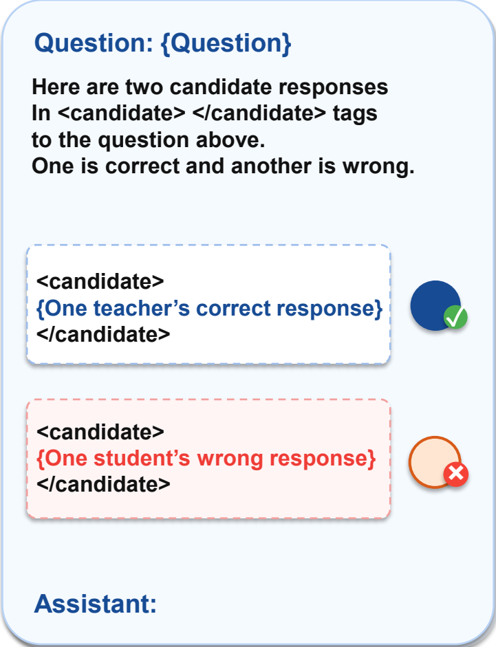
(b) Binary Candidate-included Question (BCQ)
