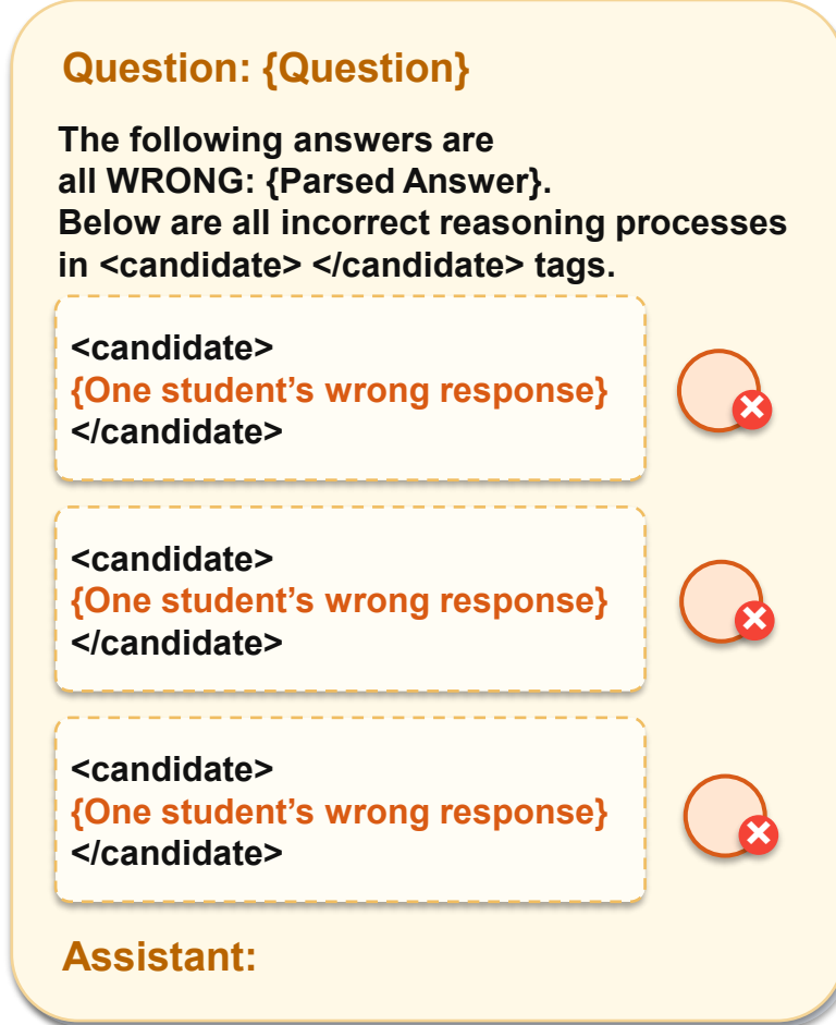
(c) Negative Candidate-included Question (NCQ)
