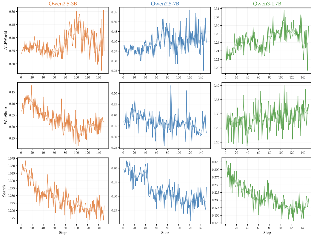
Figure 10: Gate Active Ratio when training Qwen2.5-3B, Qwen2.5-7B and Qwen3-1.7B on ALFWorld, WebShop and Search-QA.
