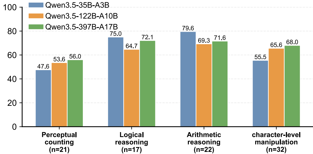
(b) Qwen series across model scales
