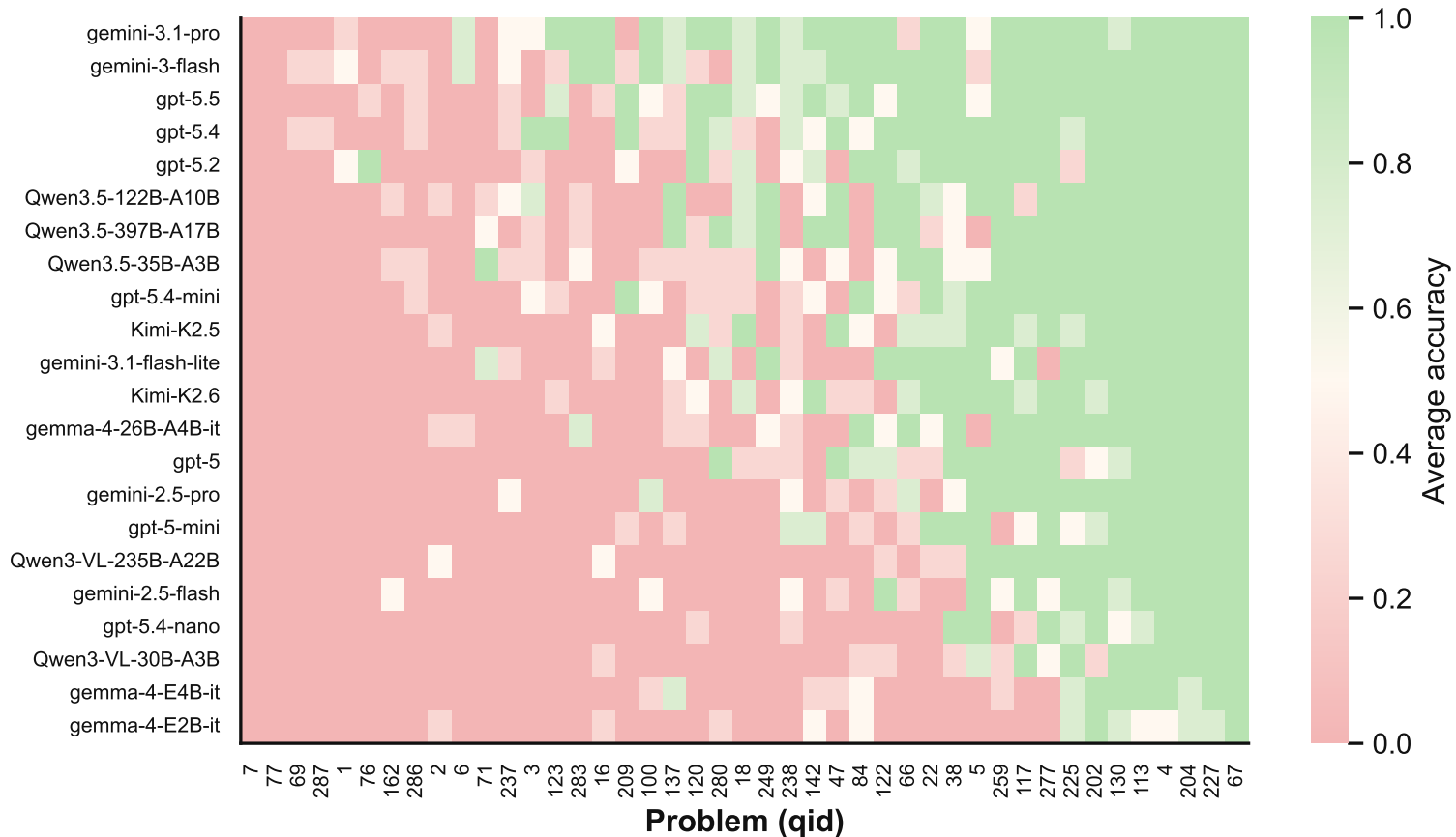
Multi-to-text Per-Problem Accuracy by Model
