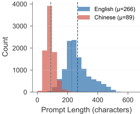
(b) Prompt Length Distribution
