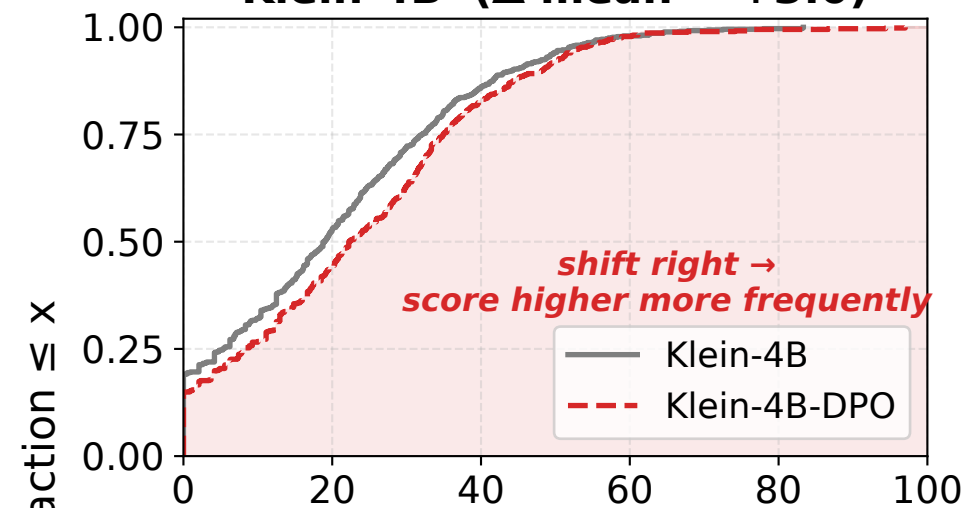
(b) Knowledge boundary shift via DPO
