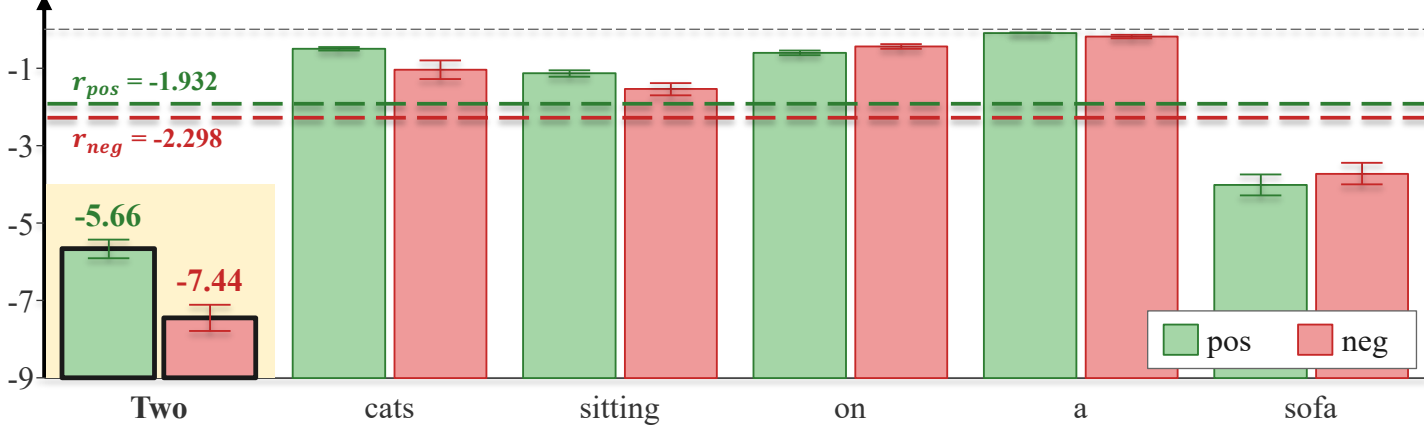
Log-Likelihood
