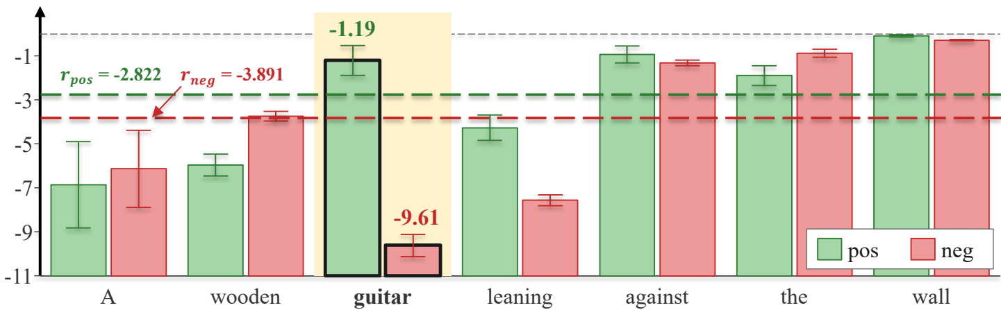
Log-Likelihood
