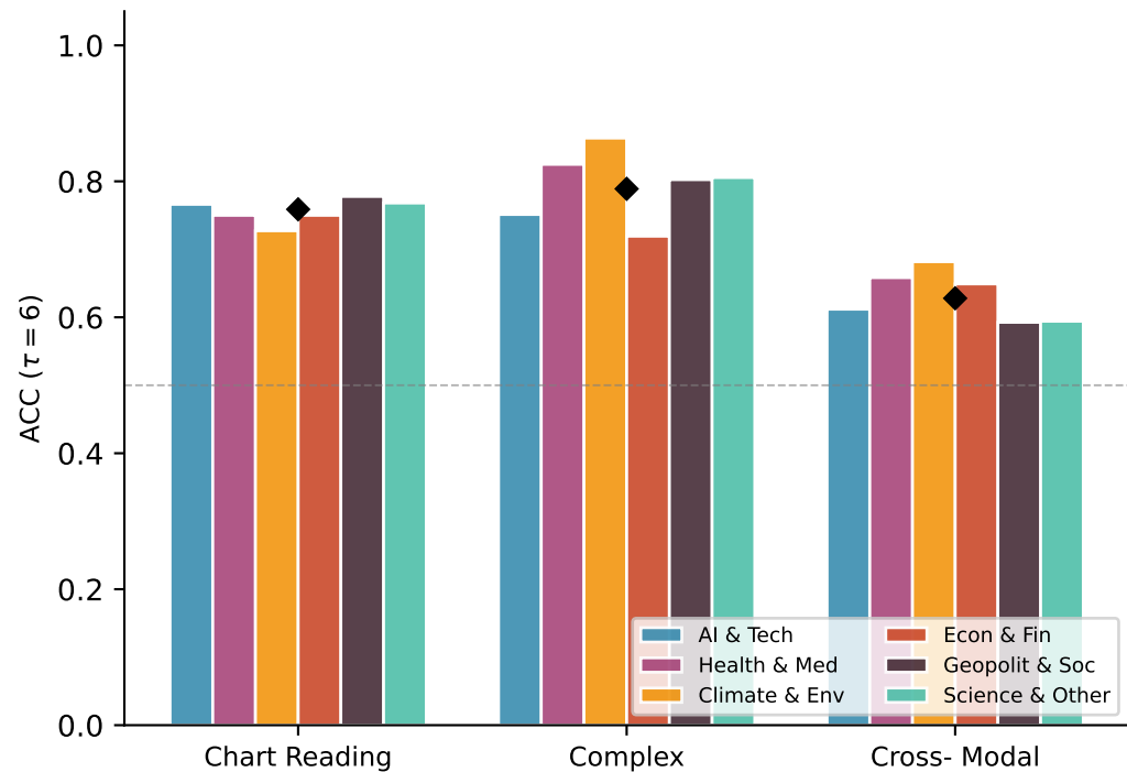
(b) Accuracy per question type
