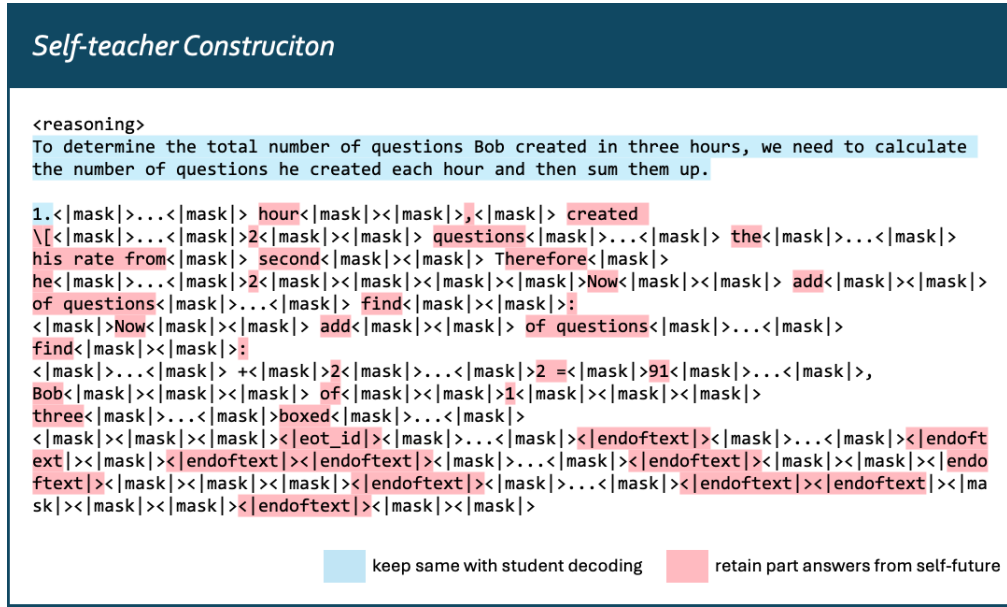
FIGURE 7 Self-teacher construction at t = 20 .
