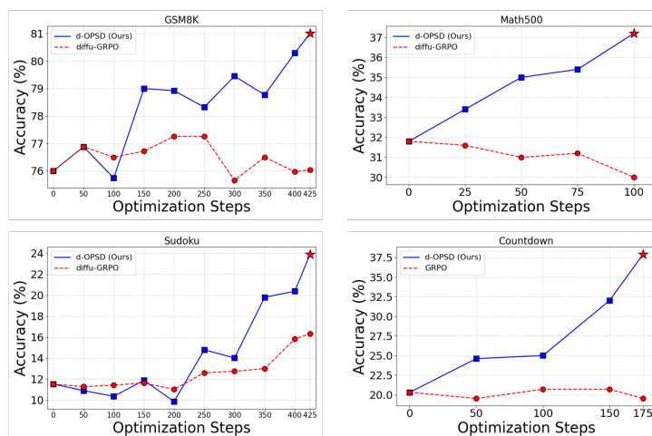
FIGURE 1 The reasoning performance and sample efficiency comparisons between the RLVR baseline (diffu-GRPO[1]) and our approach, d-OPSD.
