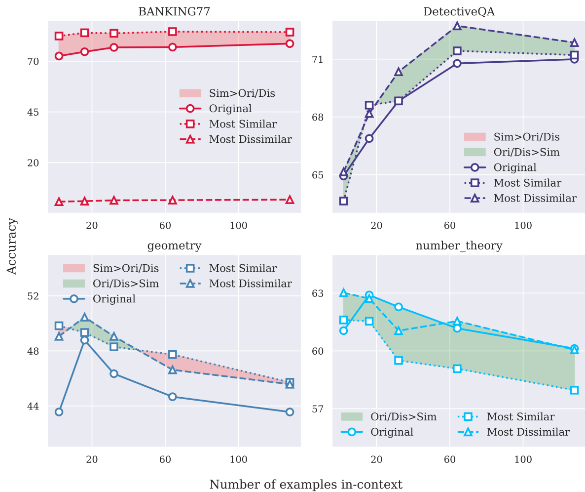
FIGURE 9 Performance with original (ori), similarity(sim) and dissimilar(dis) sets averaged across three non-reasoning LLMs . The area between the two sets is filled with colors, indicating the relative performance at each point.
