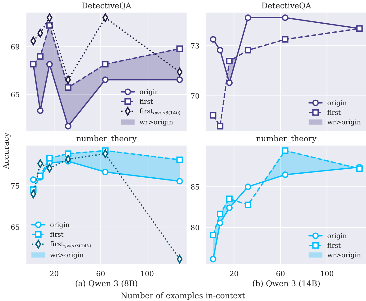
FIGURE 8 Performance of the first set of self-generated in-context CoT. \text{first}_{\text{qwen3}(14b)} is prompting the Qwen 3 (8B) model with the in-context CoT generated by Qwen 3 (14B). Left: Qwen 3 (8B) Right: Qwen 3 (14B)
