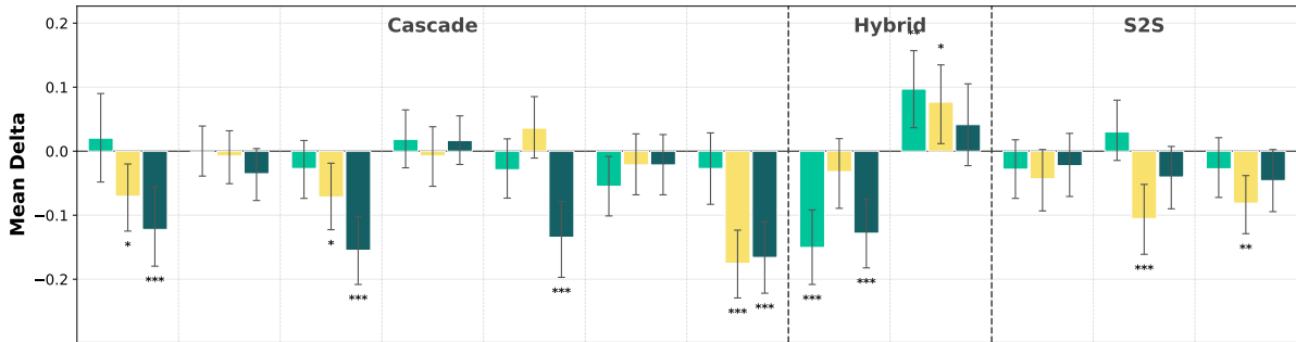
FIGURE 12 Perturbation effect on Conversation Progression across all evaluated systems, pooled across the three EVA domains. Bars show the mean delta from clean trials (negative = drop under perturbation); whiskers are 95% percentile bootstrap CIs on the per-scenario delta. Bar colors encode the perturbation condition: ■ accent, ■ background noise, ■ accent + background noise. Asterisks mark cells significant after Holm-Bonferroni correction within each model (* p < 0.05 , ** p < 0.01 , *** p < 0.001 ). Models, left to right: Cascade: Cohere – Gemma-4-26B – Voxtral, ElevenAgents (Scribe – Gemini-3-Flash – Conversational v3), Ink – Haiku-4.5 – Sonic, Nova – GPT-5.4 – Sonic, Nova – GPT-5.4-mini – Aura, Parakeet – Gemma-4-31B – Kokoro, Whisper – Qwen3.5-27B – Voxtral; Hybrid: Gemini-3-Flash – Gemini-3.1-Flash, Ultravox; S2S: Gemini-3.1-Flash-Live, GPT-Realtime-1.5, GPT-Realtime-mini.
