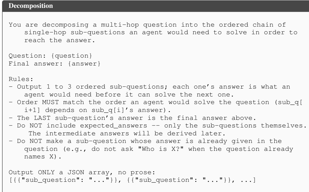
Figure 8: Tutor prompt for decomposing multi-hop questions into single-hop steps.
