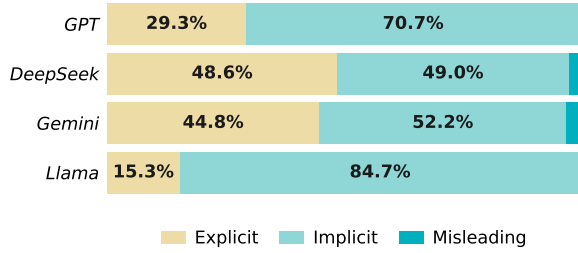
Figure 7: Distribution of invoked block alternatives under mixed blocking. For each model, the horizontal bar normalizes all invoked block alternatives to 100%. Colors indicate whether the invoked block alternative is an explicit failure, implicit failure, or semantic misleading tool. We abbreviate GPT-5.4 , Gemini-3.5-Flash , DeepSeek-V4-Flash , and Llama-3.3-70B-Instruct as GPT , Gemini , DeepSeek , and Llama .
