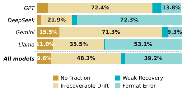
Figure 6: Trajectory Failure Category Distribution under the default setting (%). A tool call is counted as a progress call if it produces a new intermediate value required by at least one ground-truth tool-use path toward the final answer. We abbreviate GPT-5.4 , Gemini-3.5-Flash , DeepSeek-V4-Flash , and Llama-3.3-70B-Instruct as GPT , Gemini , DeepSeek , and Llama .
