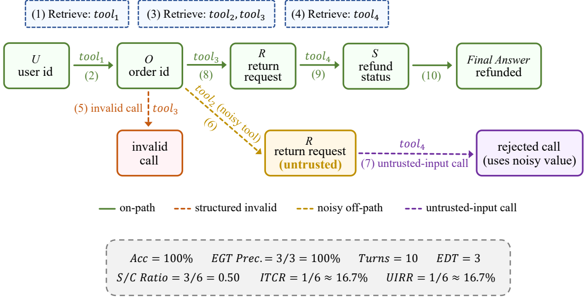
Figure 9: Illustrative trajectory for computing the seven evaluation metrics. The query starts from U and targets S along the ground-truth path U \rightarrow O \rightarrow R \rightarrow S . The agent makes one invalid call, one noisy call, and one later untrusted-input-rejected call. This trajectory yields 100% Accuracy, 100% EGT Precision, 10 turns, 3 explored datatypes, an S/C Ratio of 0.50, an ITCR of 16.7%, and a UIRR of 16.7%.
